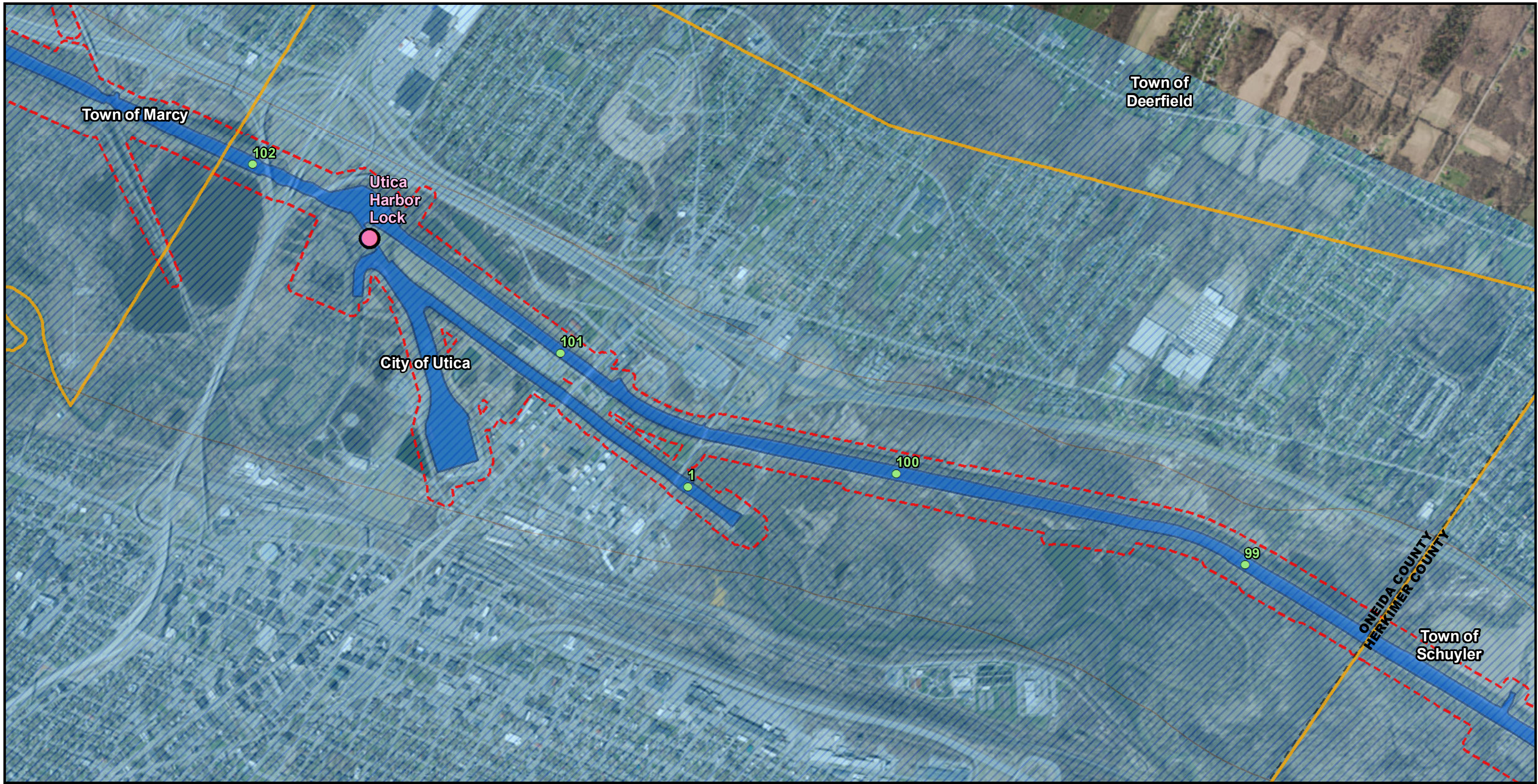
Figure 45F: Aquifers
